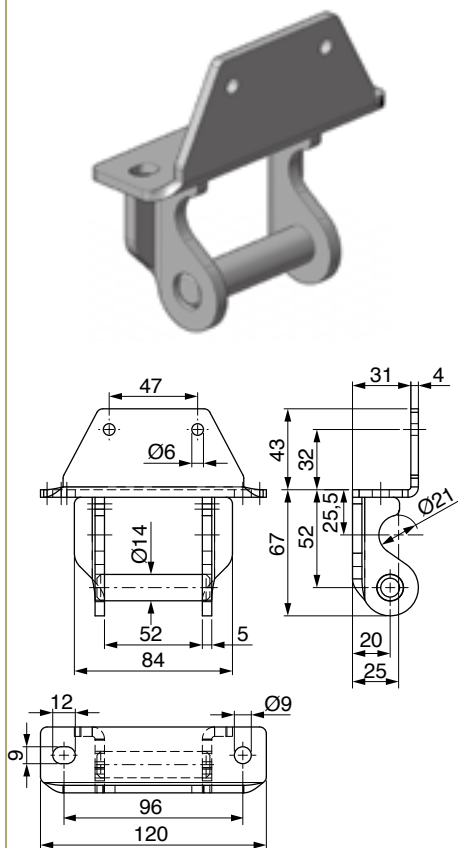
CERNIERA ZINCATA SPONDA 30mm ZINC PLATED HINGE FOR 30MM SIDEBORDS
