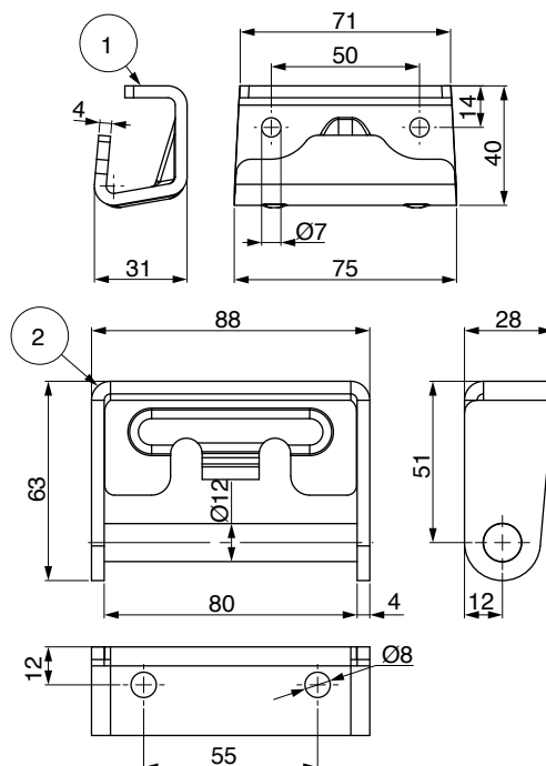
CERNIERA E SUPPORTO ZINCATI - ZINC-PLATED SUPPORT AND HINGE
