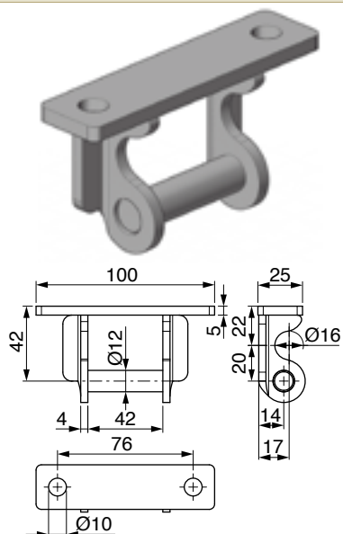
CERNIERA SPONDA ZINCATA - ZINC PLATED HINGE
