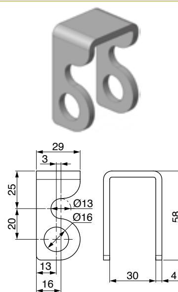
SUPPORTO BARRA - SUPPORT
