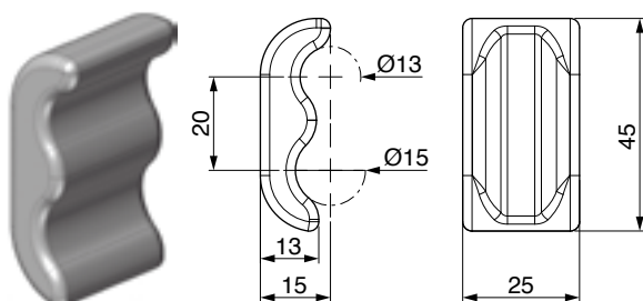
PALETTA - LOCKING PLATE
